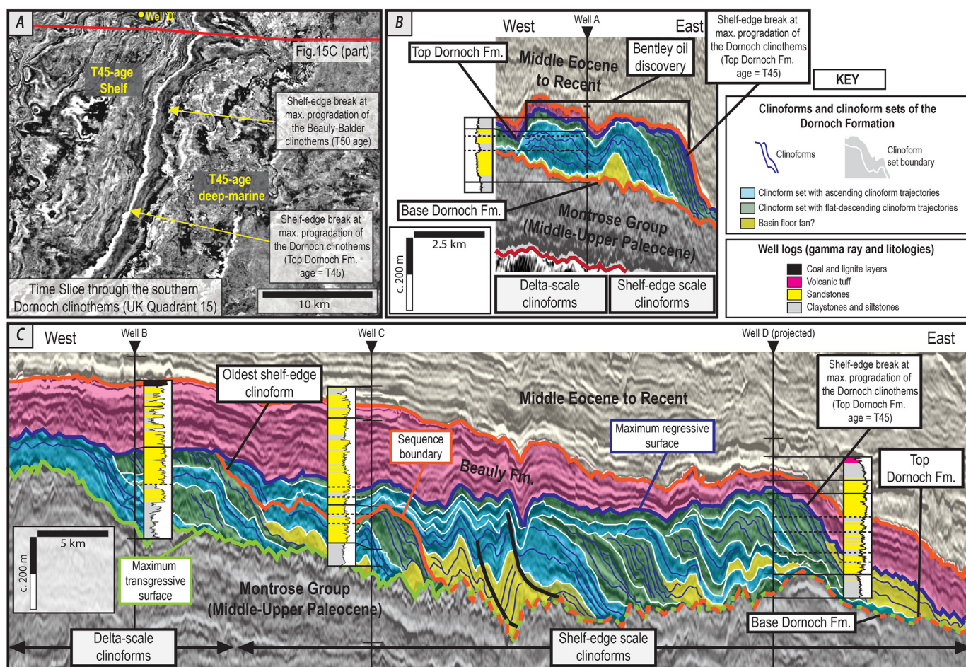
Fig. 15. Cycles of ascending and descending progradation during the outbuilding of the Dornoch Formation clinoform set (East Shetland Platform, north-eastern UK Continental Shelf) (modified after Reid and Patruno, 2015 and Patruno et al., in press). Likely basin floor fans are associated to cycles of forced regression (i.e., descending clinoform sets), with likely sequence boundaries between the two ( sensu Neal and Abreu, 2009). Because of the overall increase in accommodation during the deposition of the clinoform set, clinoforms increase their overall vertical relief from the inner to the outer part of the progradational clinoform set. As a consequence, the clinoforms evolve from delta-scale to shelf-edge scale clinoforms.
