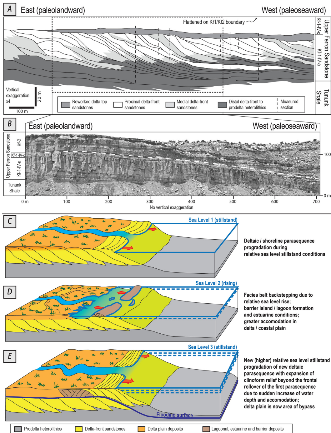
Fig. 12. (A–B) Examples of cross-sections oriented approximately parallel the depositional dip of Ancient shoreline (=subaerial delta) cliniform systems. (B) Photomosaic (no vertical exaggeration) and (A) facies interpretation (vertical exaggeration \times 4 ) of a cliff face (along depositional dip) of the Cretaceous-age Ferron Sandstone ancient shoreline cliniform system (Ivie Creek amphitheatre, Utah, U.S.A.) (after Anderson et al., 2002 and Gani and Bhattacharya, 2005). (C–E) Sketches illustrating the evolution of an idealised wave-dominated shoreline through times, forming a succession of progradational cliniform sets, each deposited during phases of relative sea-level stillstand and stacked on top of each other due to the episodic transgressive backstepping of the coastal system (redrafted after Howell and Flint, 2002b).
