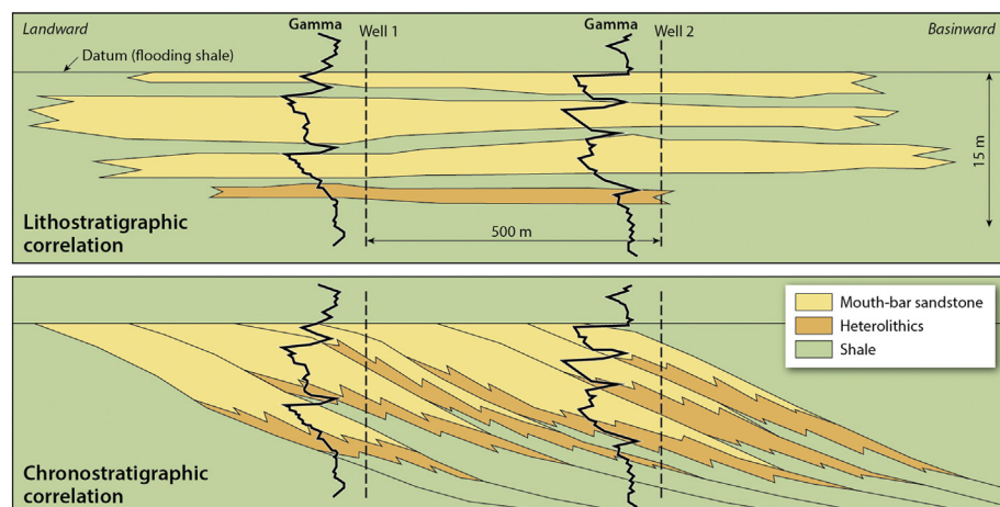
Fig. 4. Comparison between lithostratigraphic and chronostratigraphic correlations (modified after Ainsworth et al., 1999 and Gani and Bhattacharya, 2005). The chronostratigraphic correlation relies on clinoform-shaped time-lines that approximate the “real” depositional morphology and three-dimensional sedimentary architecture of clinothem.
